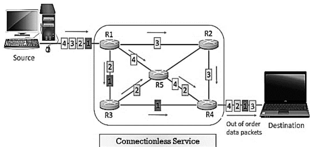
Figure 10. 9 Connectionless Service
