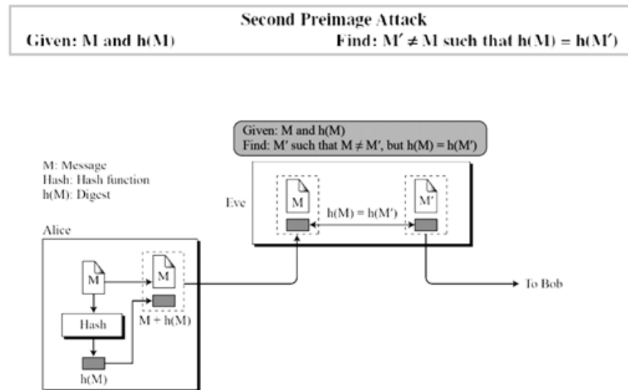
Figure: Second preimage
