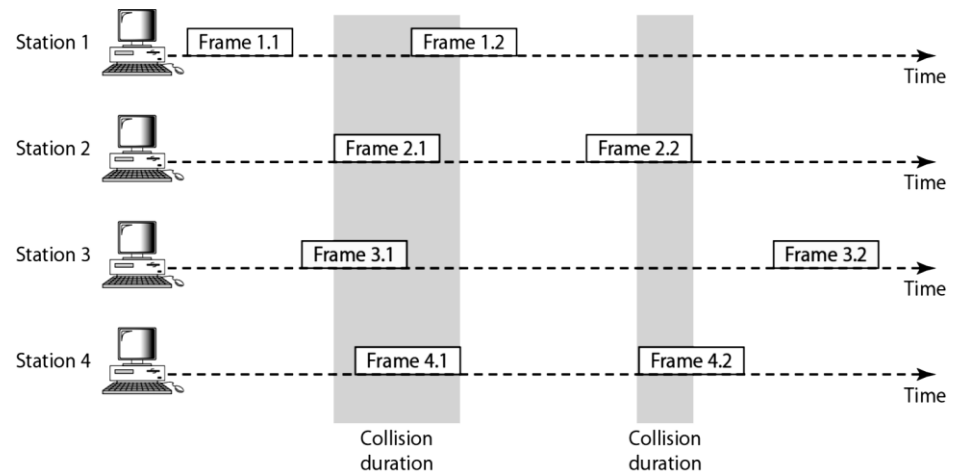
Figure 7.4 A scenario of Collisions
