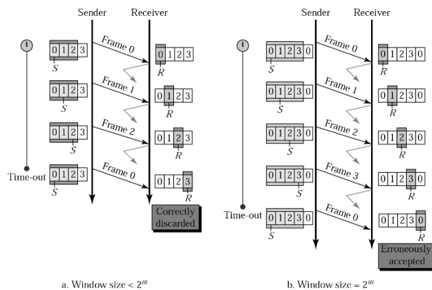
Figure 6.24 Sender Window Size
