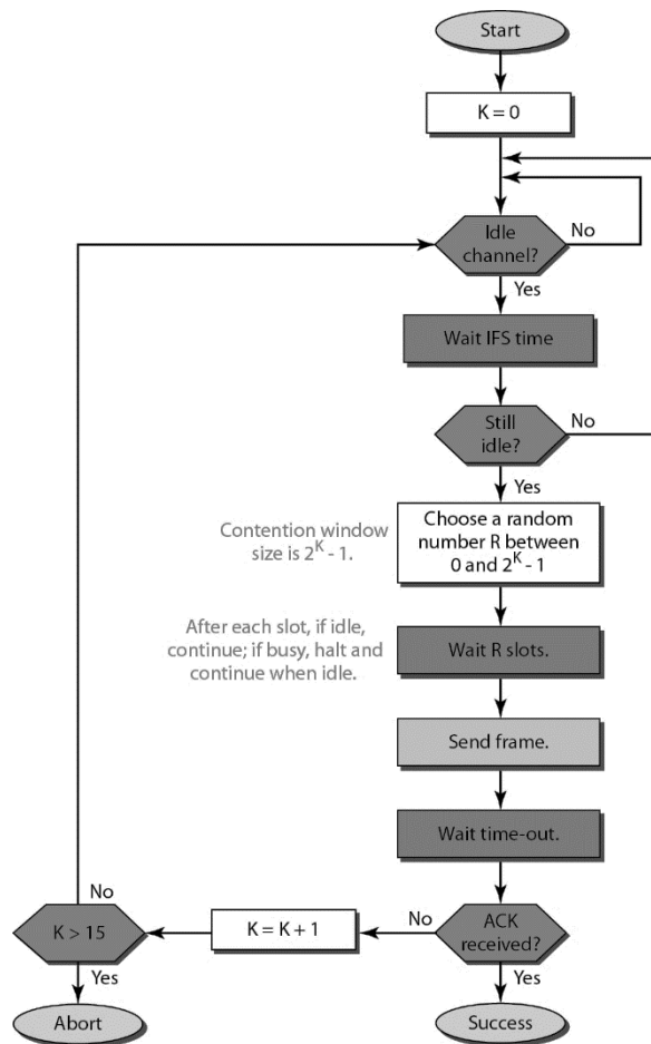
Figure 7. 18 Flow Chart of Carrier Sense Multiple Access with Collision Avoidance
