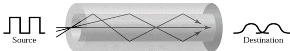
Figure 4. 15 Multimode, Step Index
