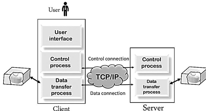
Figure 12.5 Mechanism of FTP
