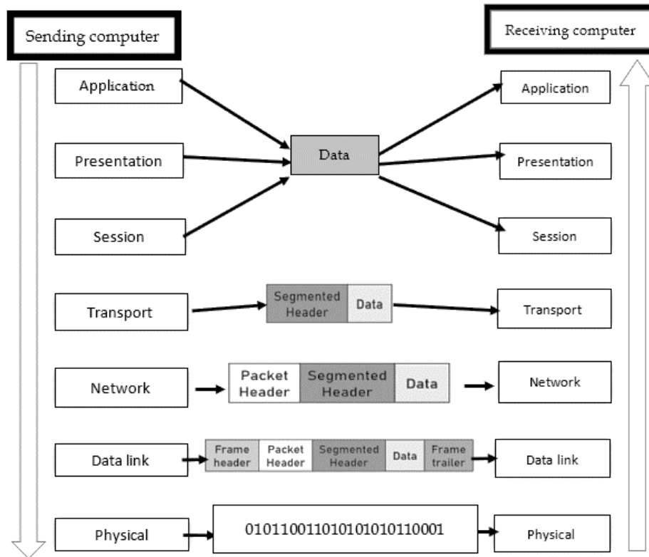
Figure 3.5 Encapsulation &amp; De-encapsulation in OSI Model
