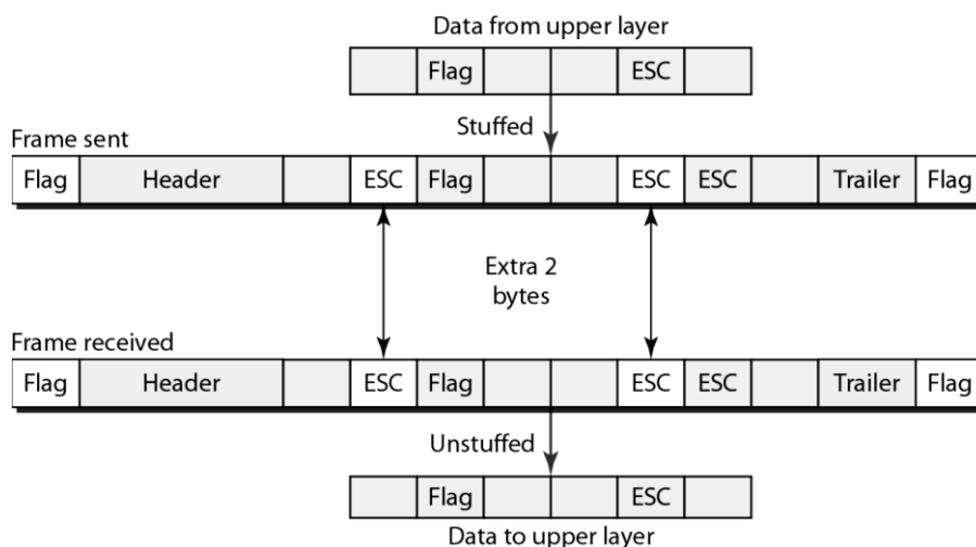
Figure 5.7(a) Byte Stuffing and Unstuffing
