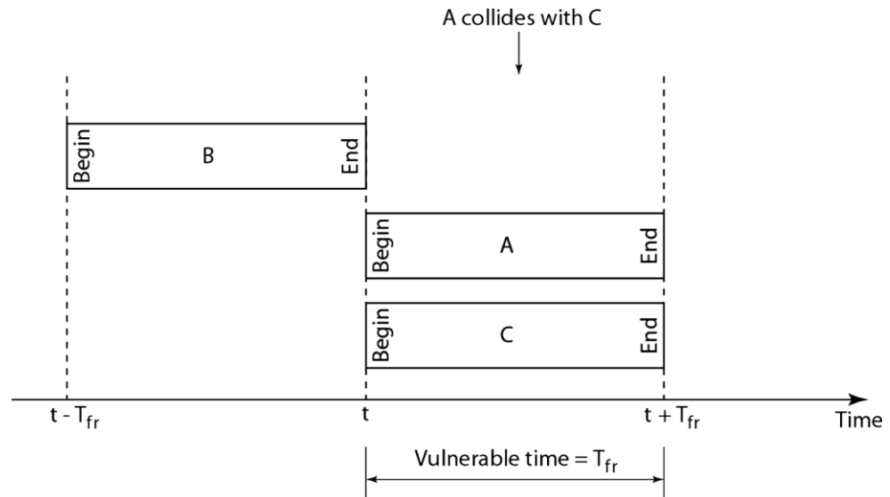
Figure 7. 8 Slotted ALOHA vulnerable time = T_{fr}
