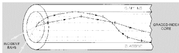
Figure 4. 16 Multimode Graded Index
