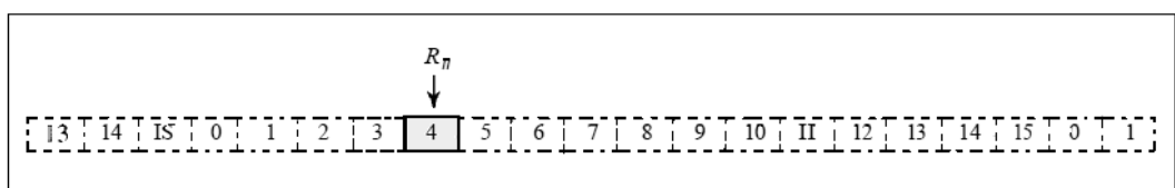
Figure 6.18 (a) The receive window.
