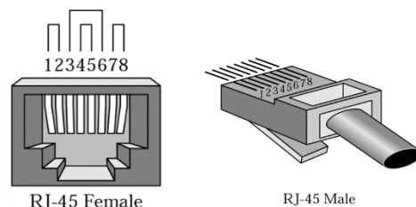
Figure 4. 7 RJ45 Connectors
