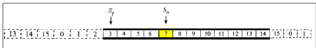
Figure 6.17 Send Window After Sliding
