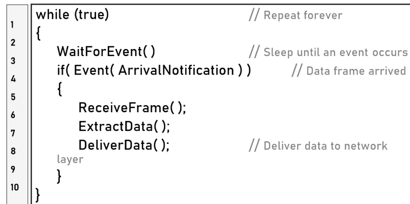
Figure 6.4 Receiver-site Algorithm for the Simplest Protocol
